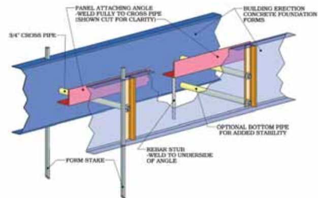
Figure 4 - Building Erection Concrete Foundation Forms
