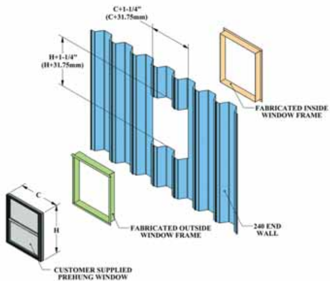
Window Cutout and Installation
