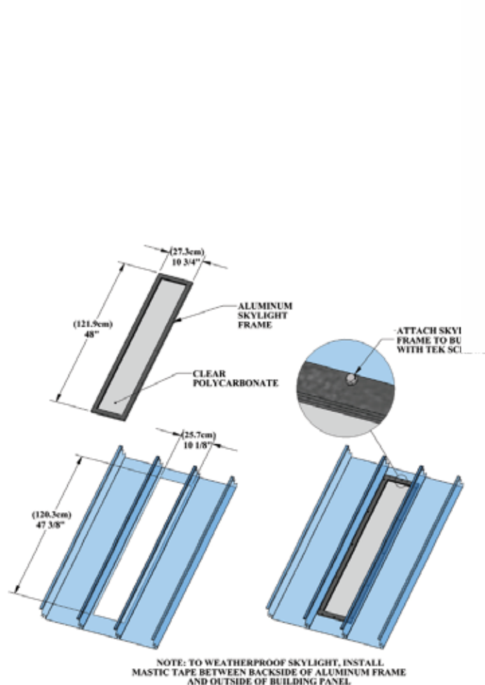
Skylight Installation
