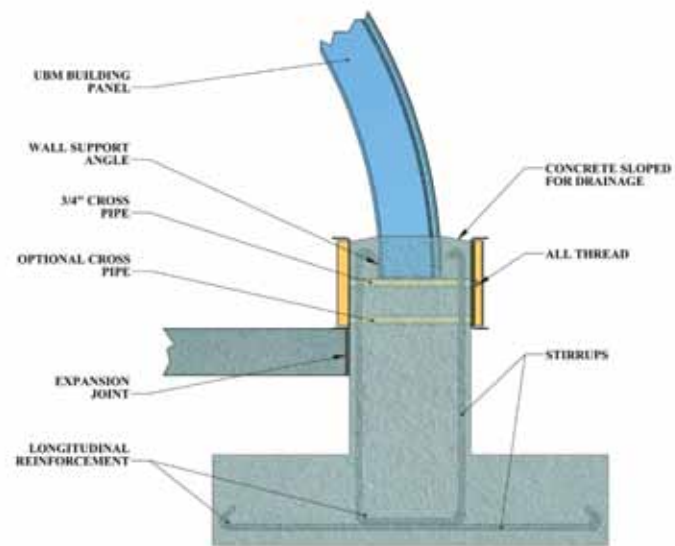
Concrete Foundation Front View (Spread)
