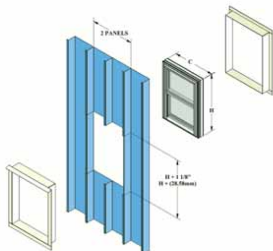
Window Cutout and Installation
