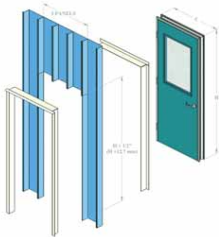
Door Cutout and Installation
