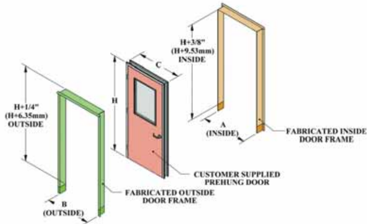
Typical Door Frame
