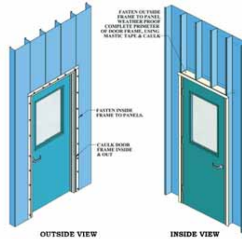
Typical Door Views
